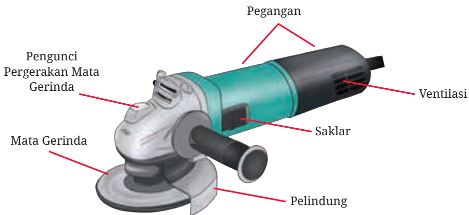
Gambar 4.24 Gerinda ( Angle Grinder ) Sumber: Eko Arianto (2022)
