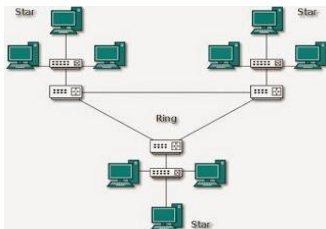
Gambar Topologi Hybrid
